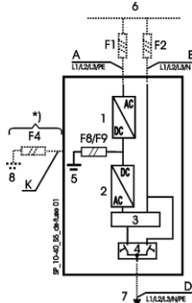
Separated input Rectifier & Bypass (recommended)
