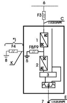
Common input Rectifier & Bypass
